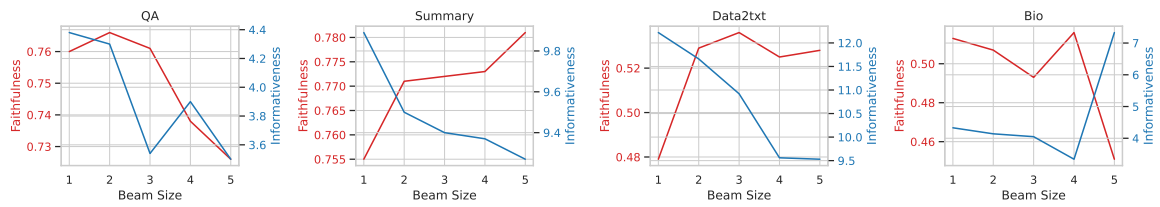
Figure 6: Faithfulness and Informativeness of Llama 2 7B Chat as a function of the beam size.
