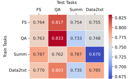
Figure 4: Performance of \text{SYNCHECK}_{\text{MLP}} on different train-test task pairs using Llama 2 7B Chat. We report the AUROC averaged across three runs.
