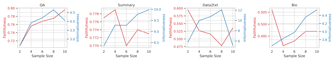
Figure 7: Faithfulness and Informativeness of Llama 2 7B Chat as a function of the sample size.
